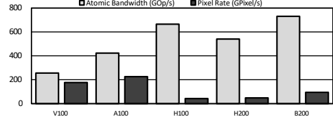
Fig. 8: ROP bandwidth over GPU generations: In AI-focused GPUs (H100, H200, and B200), ROP (atomic) bandwidth scales while graphics (pixel) throughput significantly declines.
